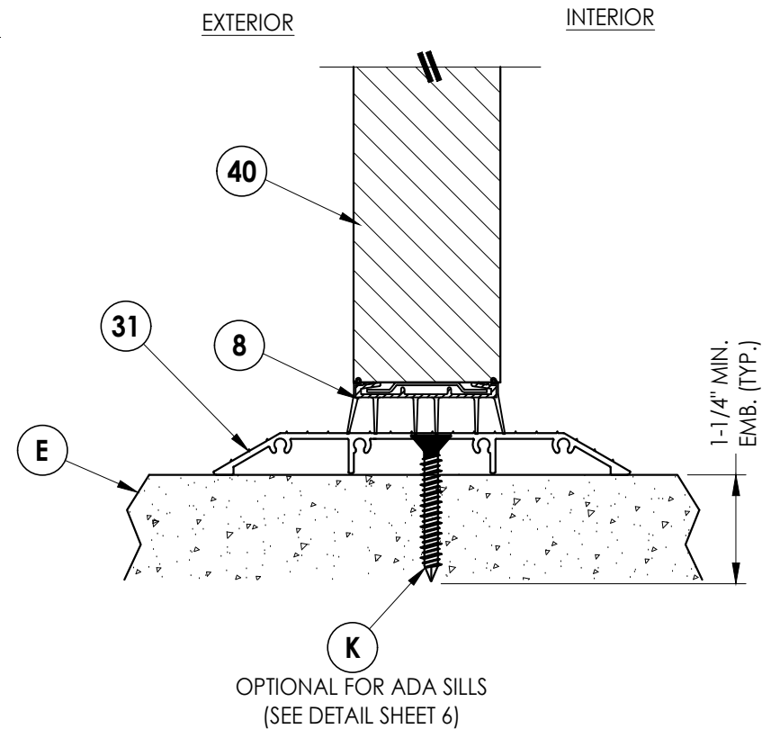
3 5 VERTICAL CROSS SECTION
