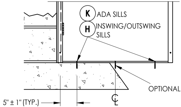
OPTIONAL SILL ANCHORING IN LIEU OF FRAME CORNER CONNECTIONS (SEE CORNER DETAIL - SHEET 3)
