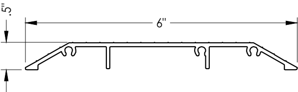
31 ADA THRESHOLD AFCO A-202
